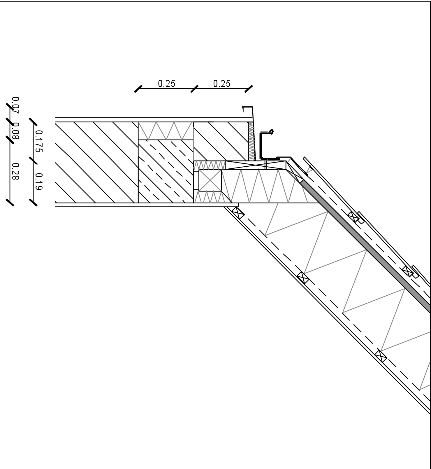
Detail Traufe M 1: 10
